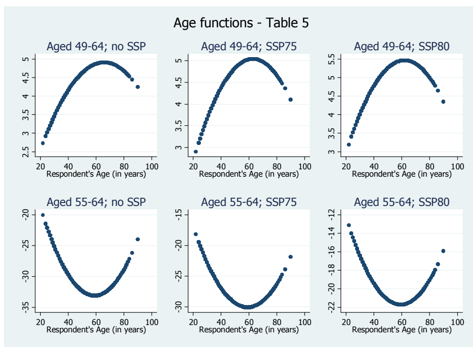
Figure 3: Age functions associated to the regressions in Table 5.
